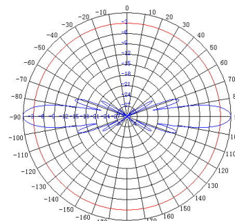
E Plane
